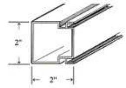
H122 - Vertical supports
