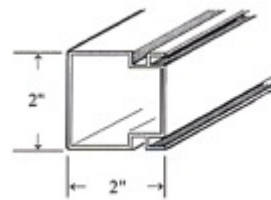
H122 - Vertical supports
