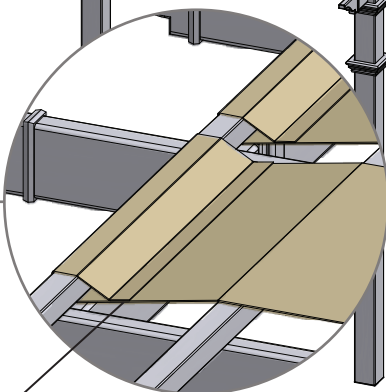
End of canvas wraps around the end shade slat as shown.
